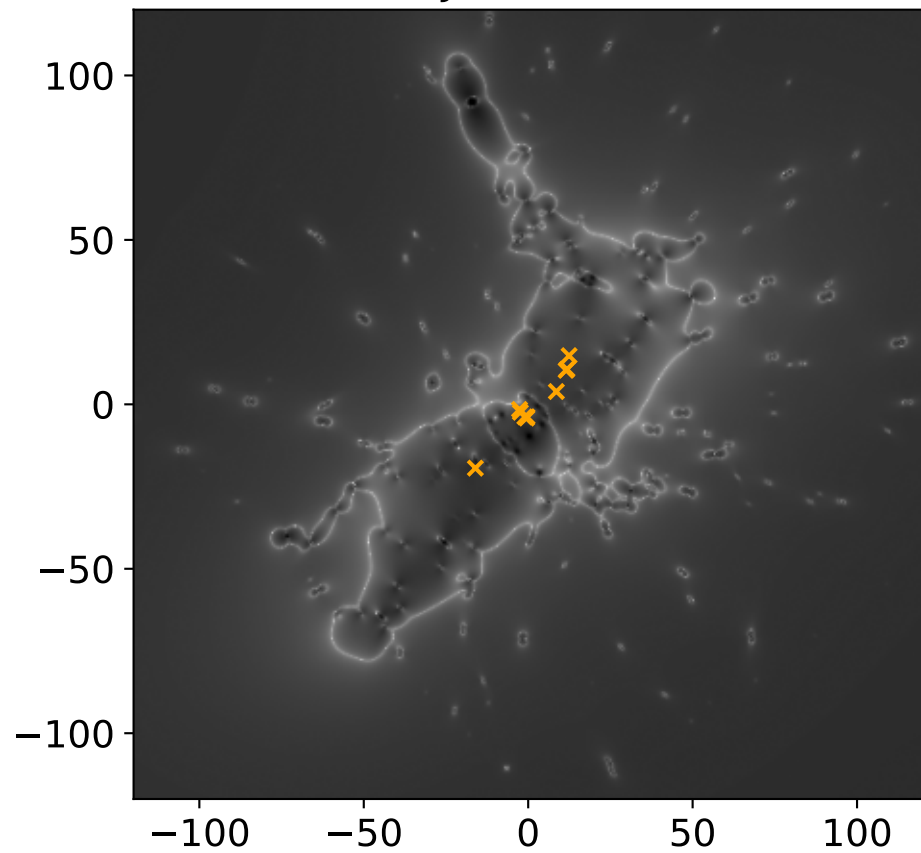
MACS J1149.5+2223
